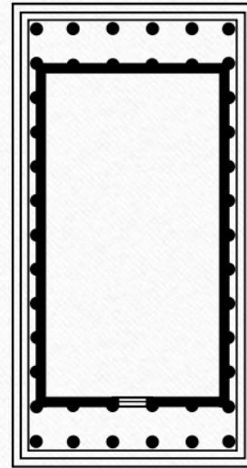
pseudoperipteral
